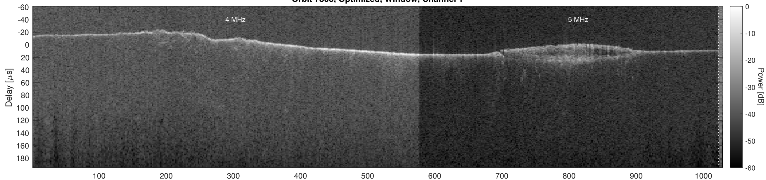
Orbit 7803, Optimized, Window, Channel 2
