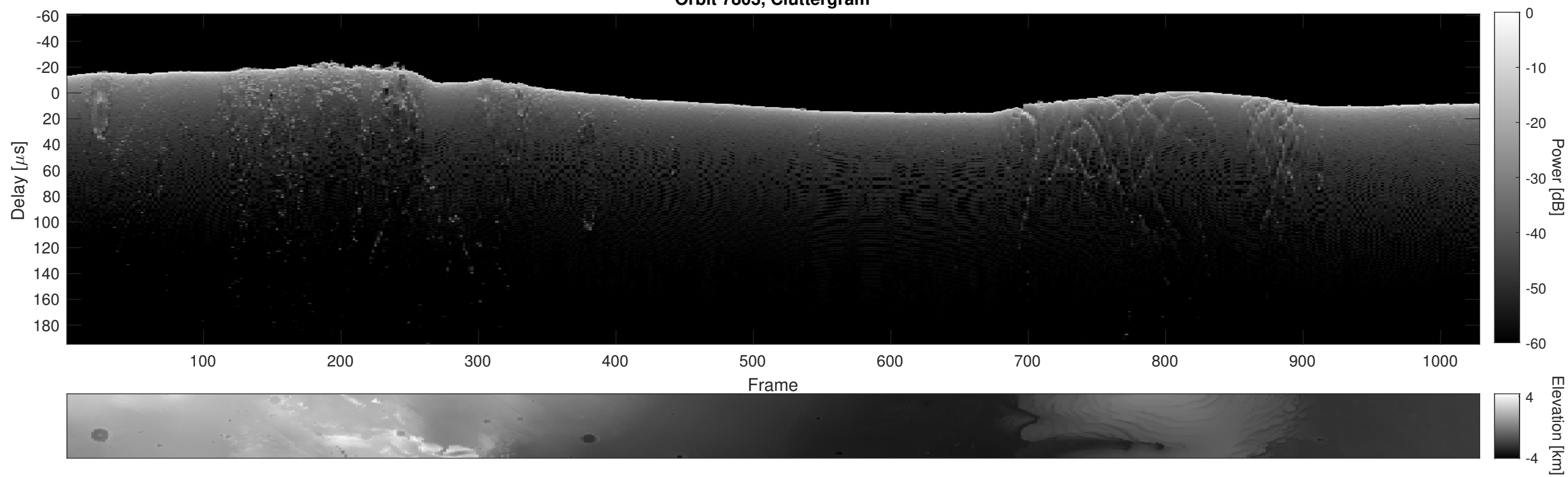
Orbit 7803, Cluttergram
