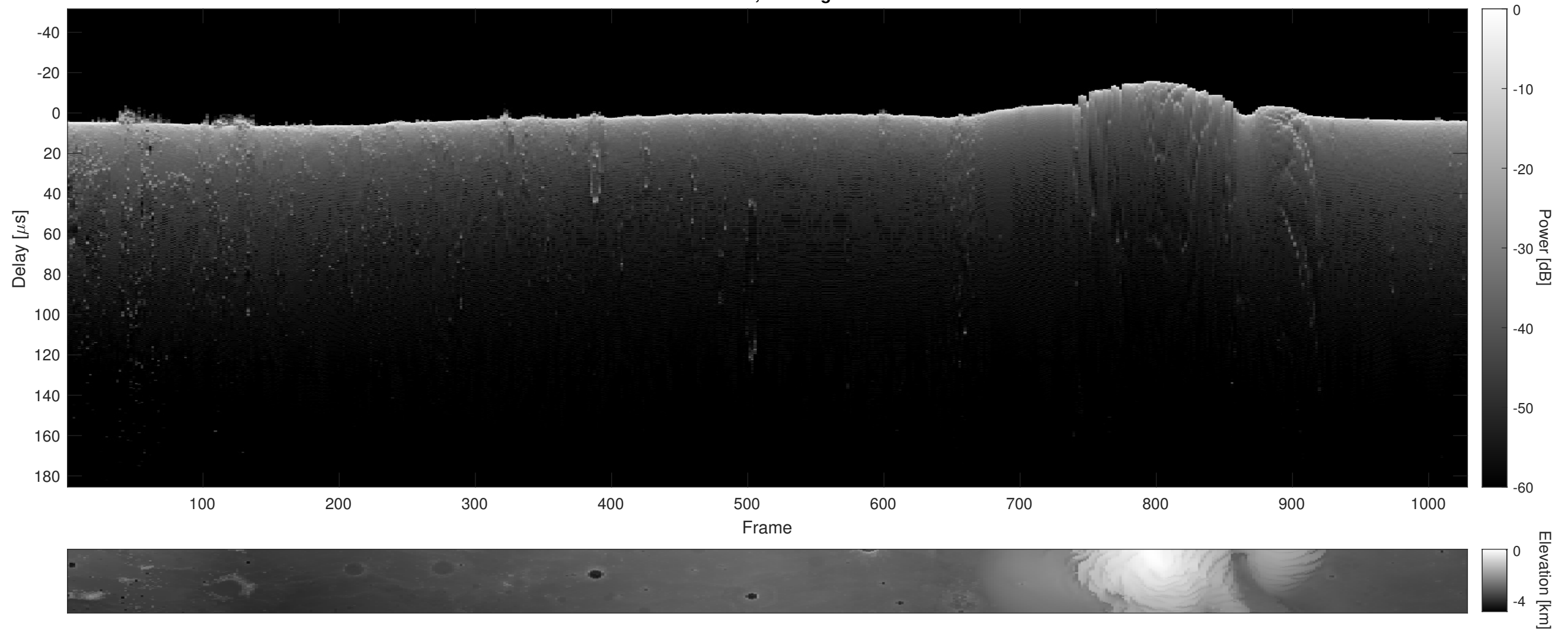
Orbit 7804, Cluttergram
