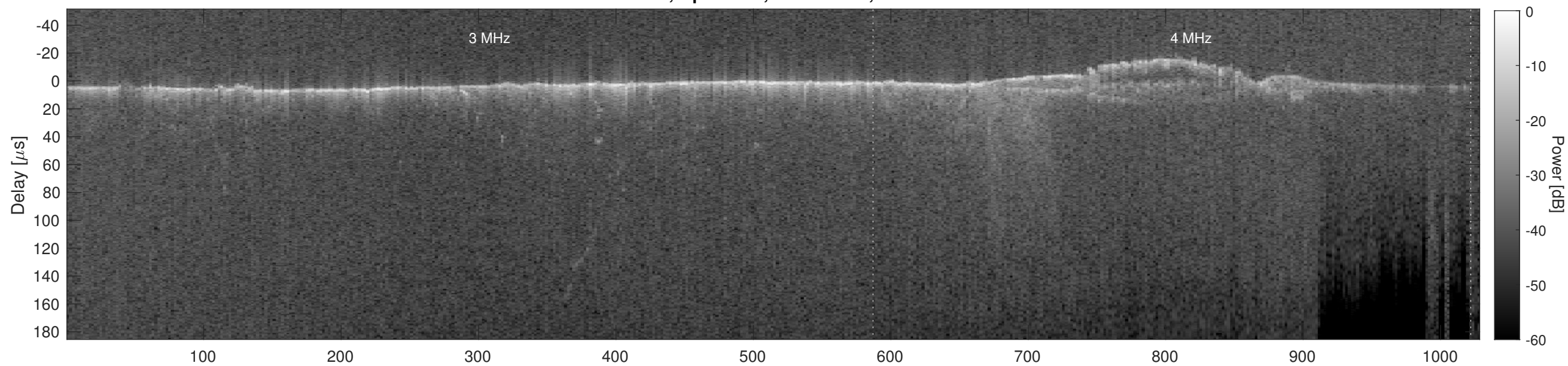
Orbit 7804, Cluttergram
