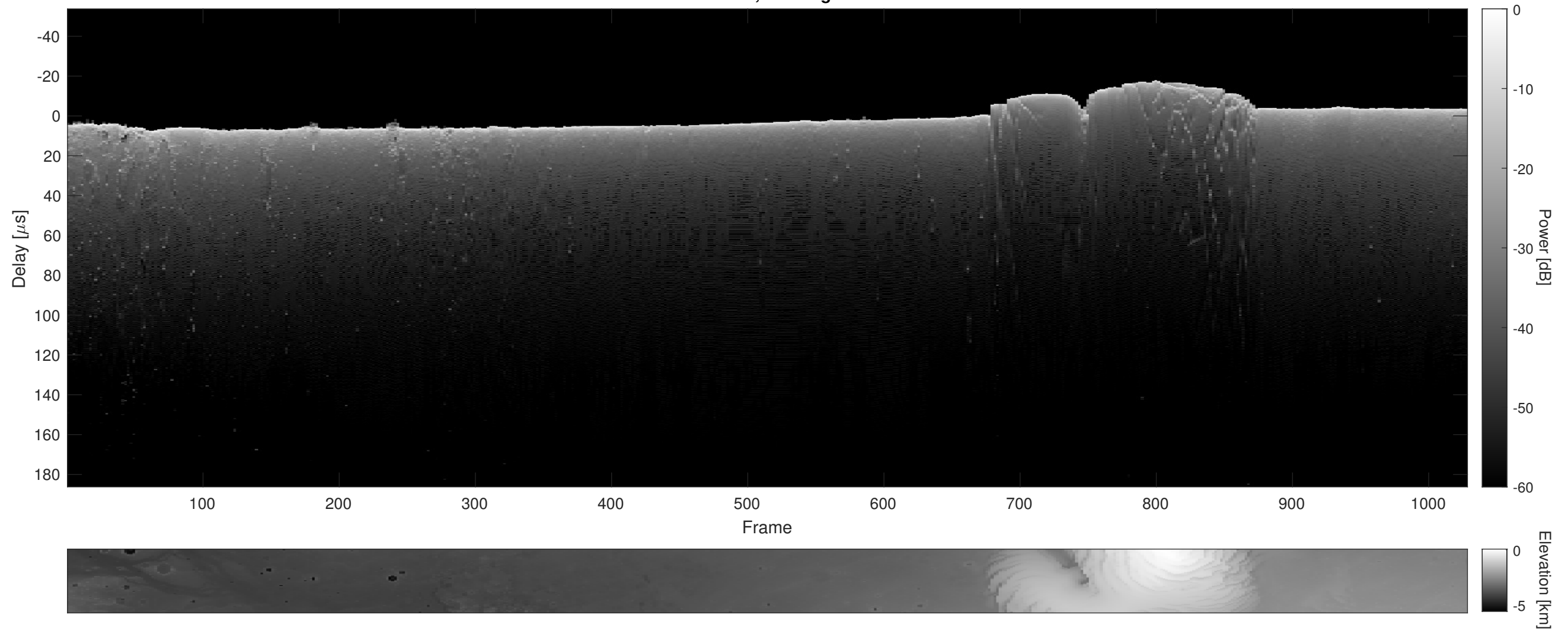
Orbit 7806, Cluttergram
