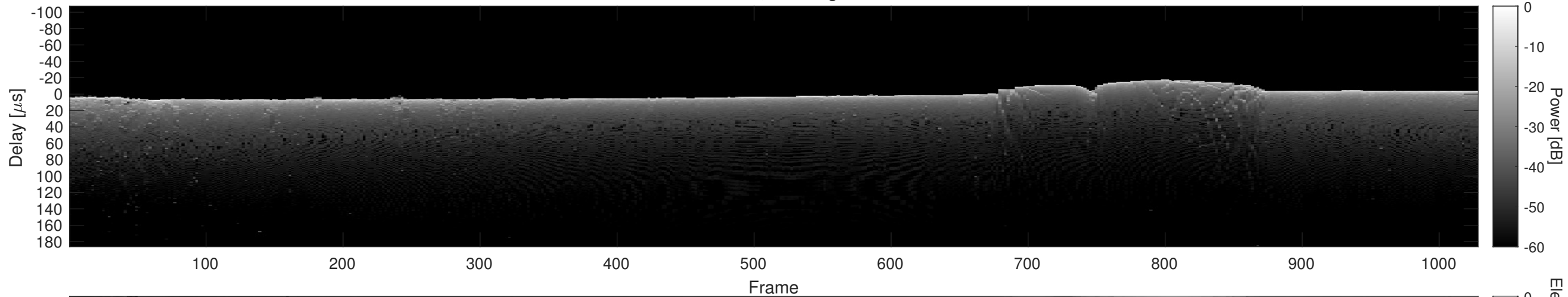
Orbit 7806, Cluttergram
