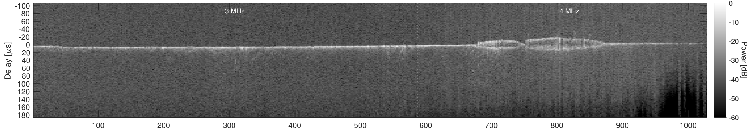
Orbit 7806, Cluttergram
