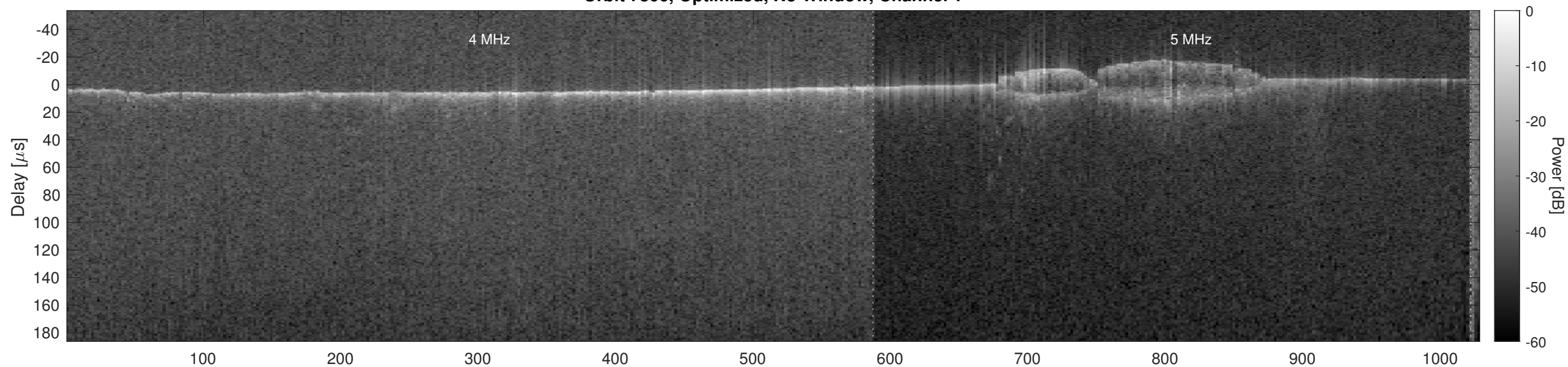
Orbit 7806, Optimized, No Window, Channel 2
