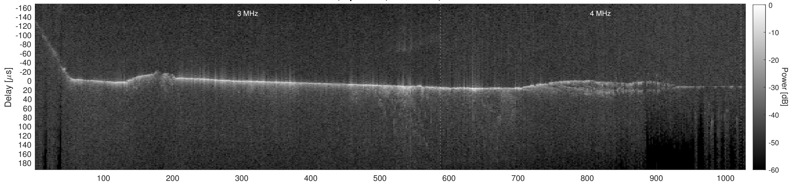
Orbit 7807, Cluttergram
