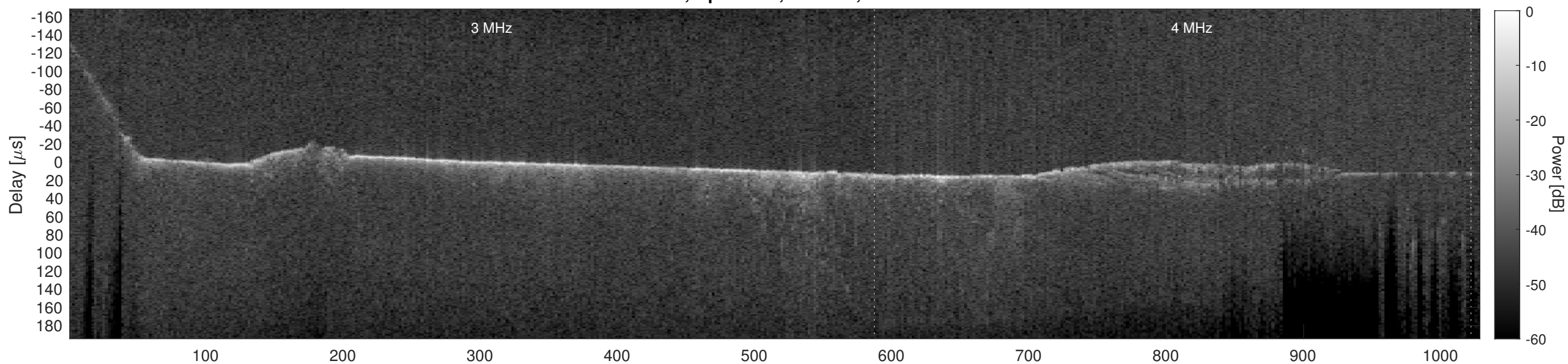
Orbit 7807, Cluttergram
