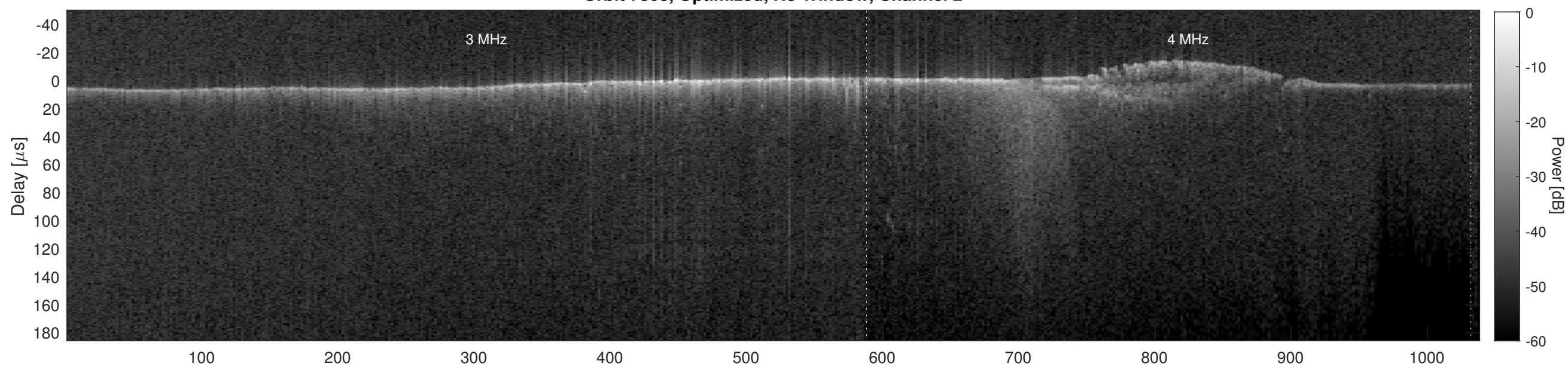
Orbit 7808, Cluttergram
