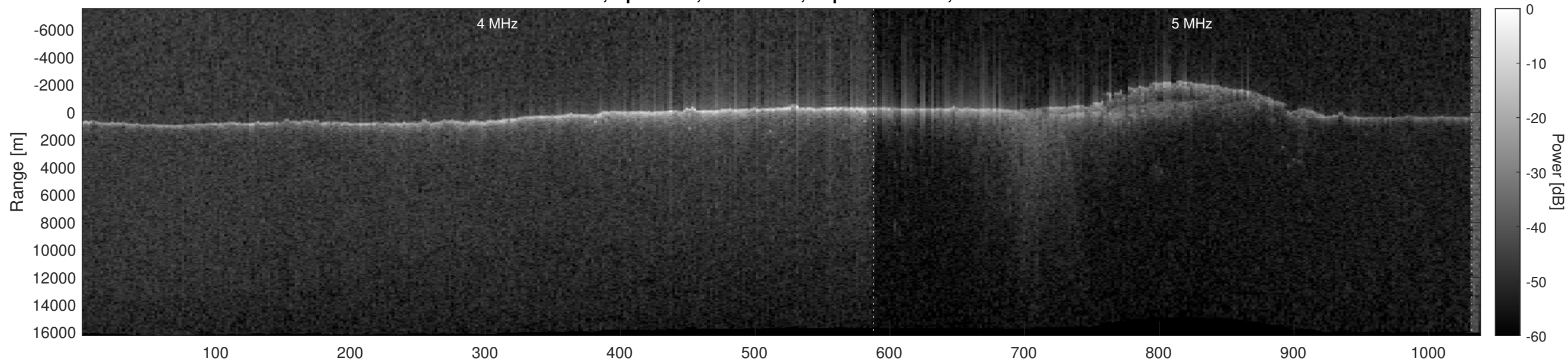
Orbit 7808, Optimized, No Window, Depth-Corrected, Channel 2
