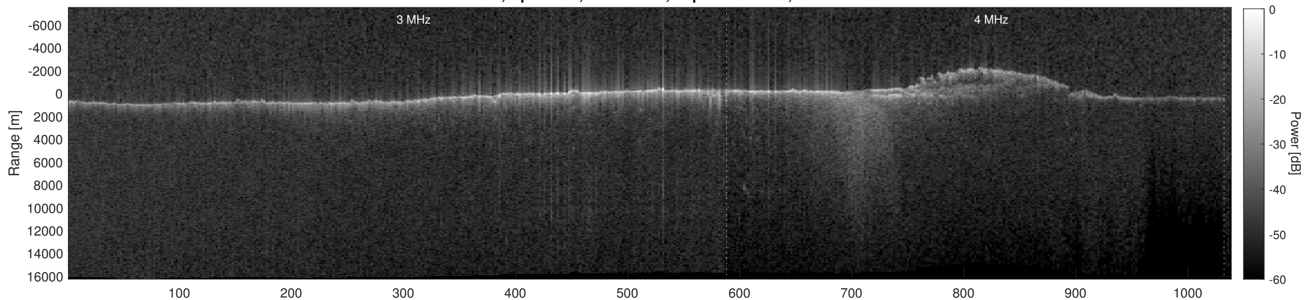
Orbit 7808, Depth-Corrected Cluttergram
