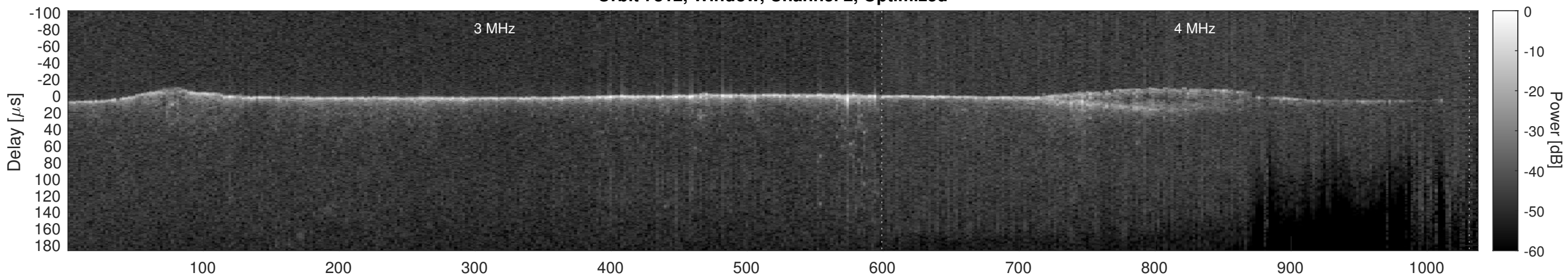
Orbit 7812, Cluttergram
