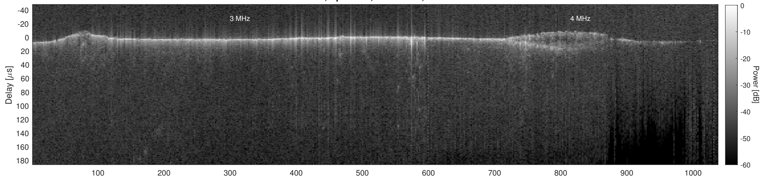
Orbit 7812, Cluttergram
