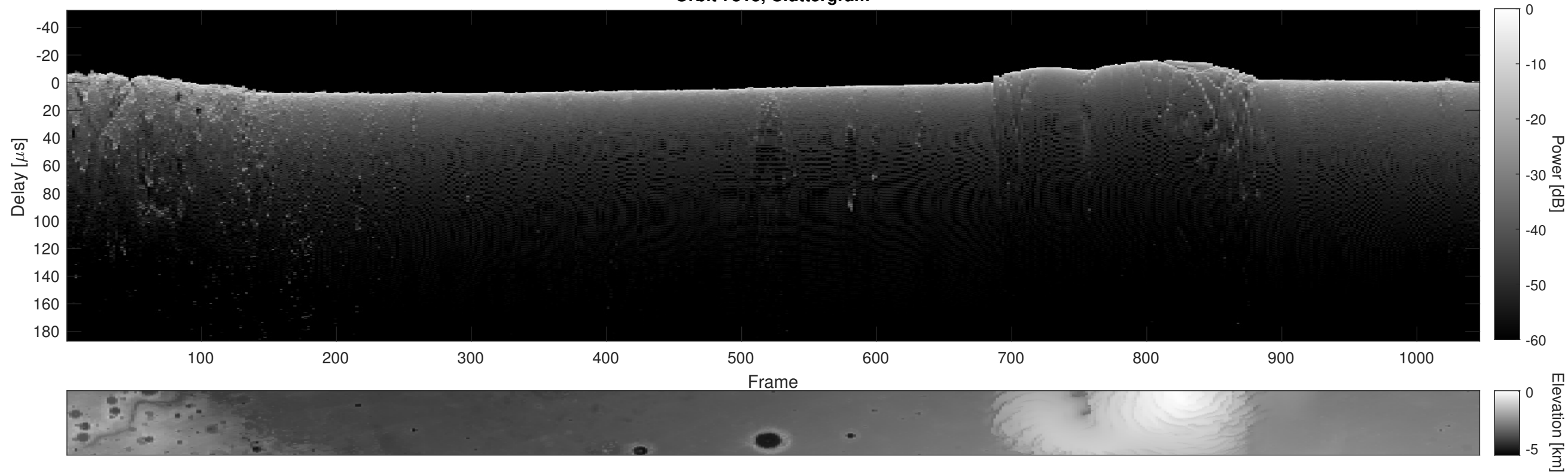
Orbit 7813, Cluttergram
