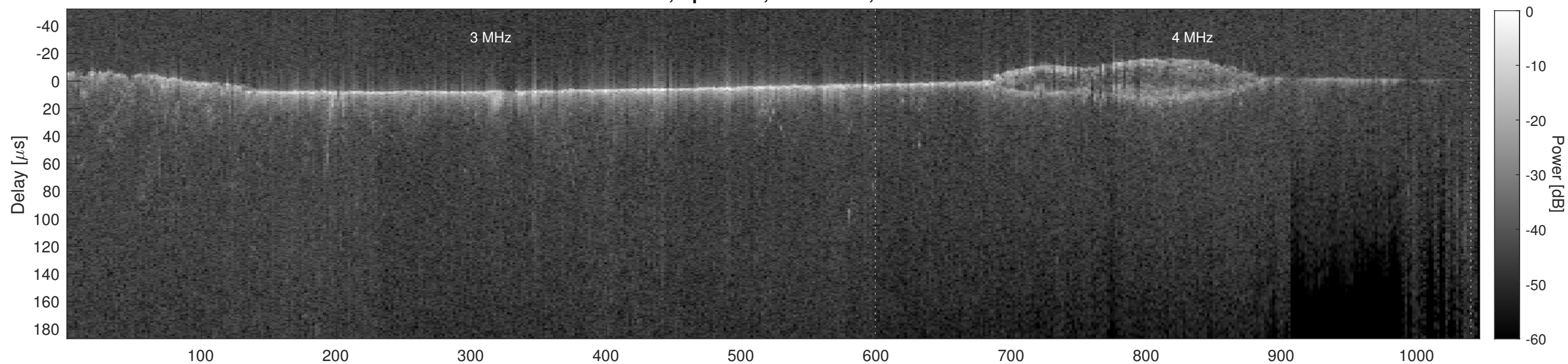
Orbit 7813, Cluttergram
