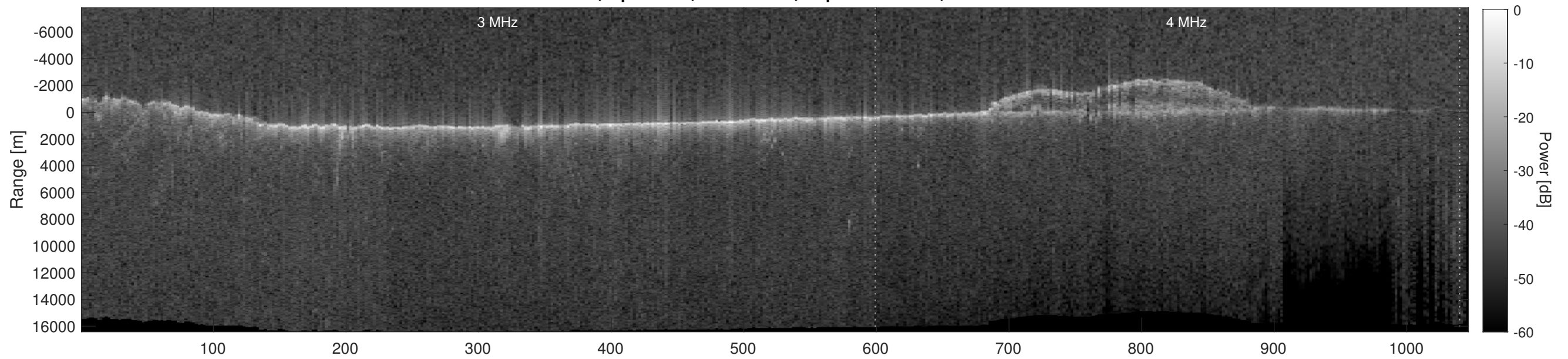
Orbit 7813, Depth-Corrected Cluttergram
