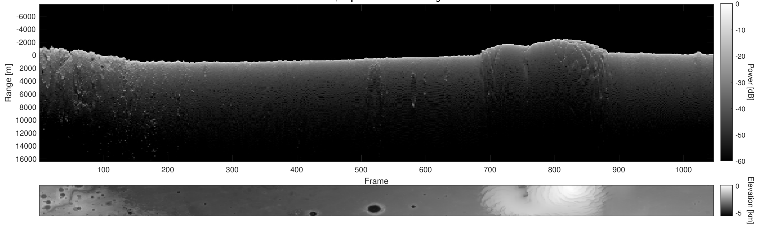
Orbit 7813, Depth-Corrected Cluttergram
