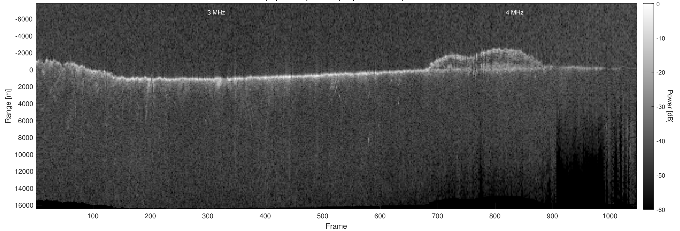
Orbit 7813, Optimized, Window, Depth-Corrected, Channel 2
