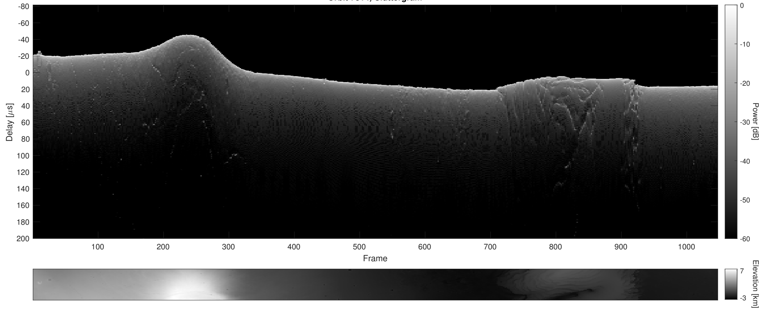
Orbit 7814, Cluttergram
