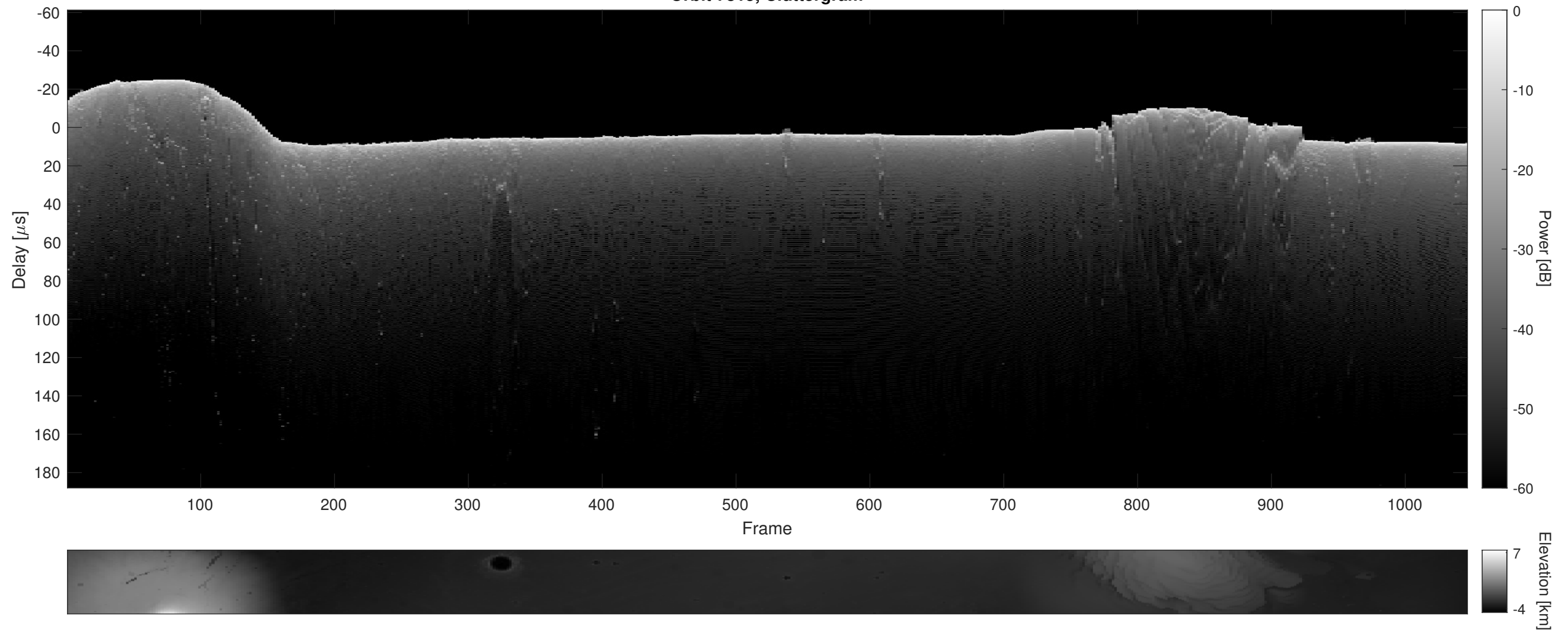
Orbit 7815, Cluttergram
