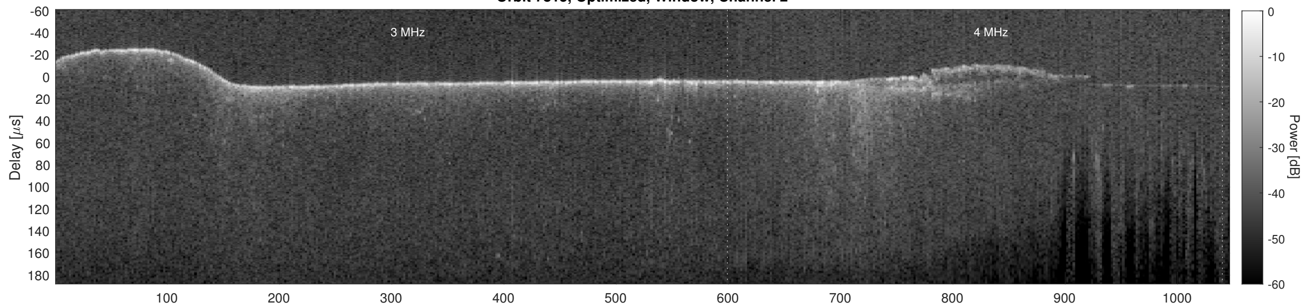
Orbit 7815, Cluttergram
