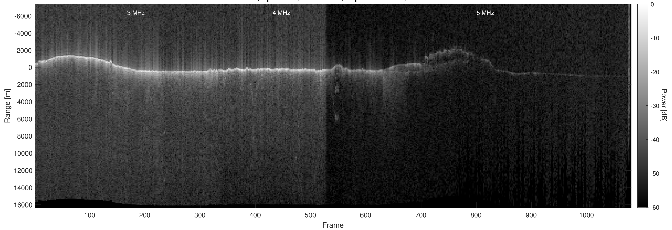
Orbit 7822, Optimized, No Window, Depth-Corrected, Channel 2
