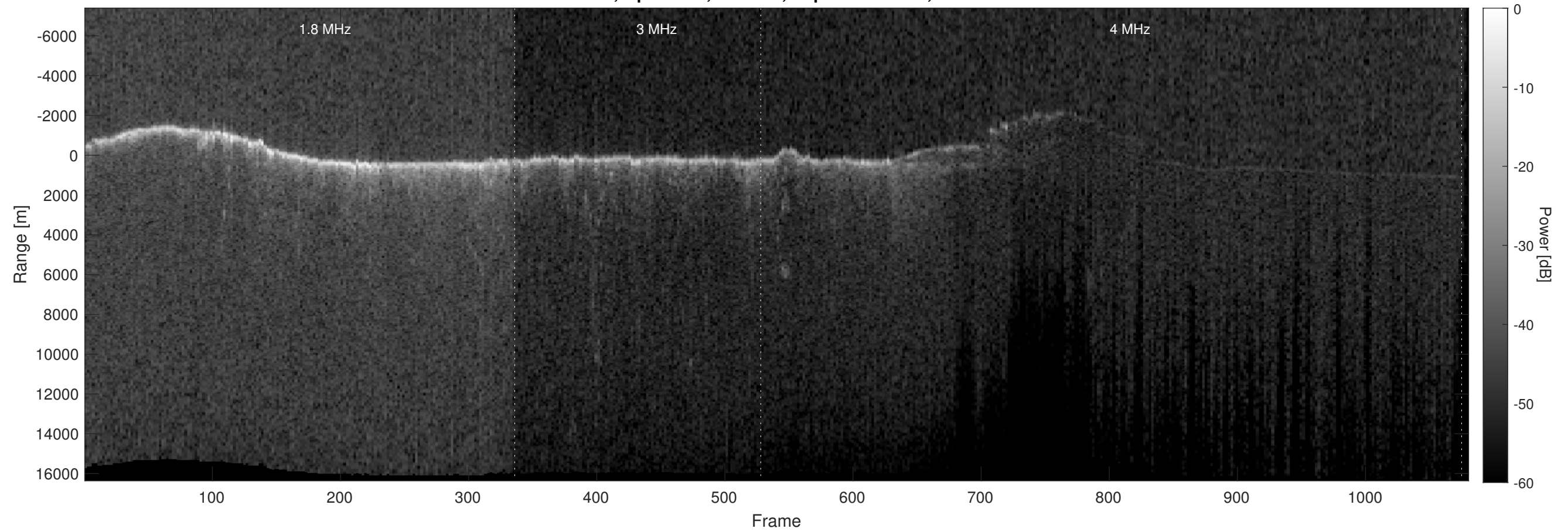
Orbit 7822, Optimized, Window, Depth-Corrected, Channel 2
