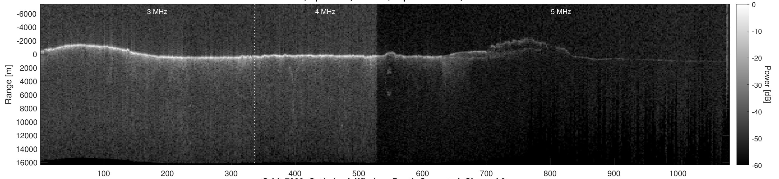
Orbit 7822, Optimized, Window, Depth-Corrected, Channel 2
