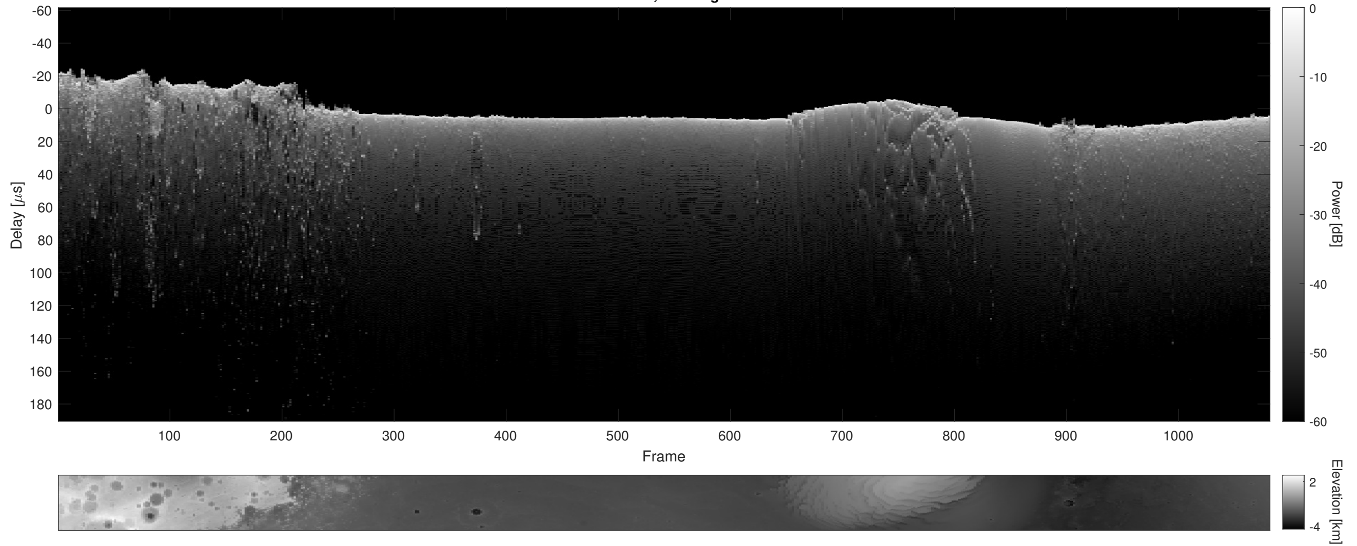
Orbit 7823, Cluttergram
