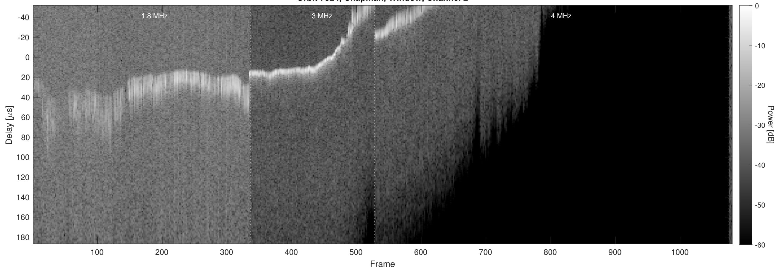
Orbit 7824, Chapman, Window, Channel 2
