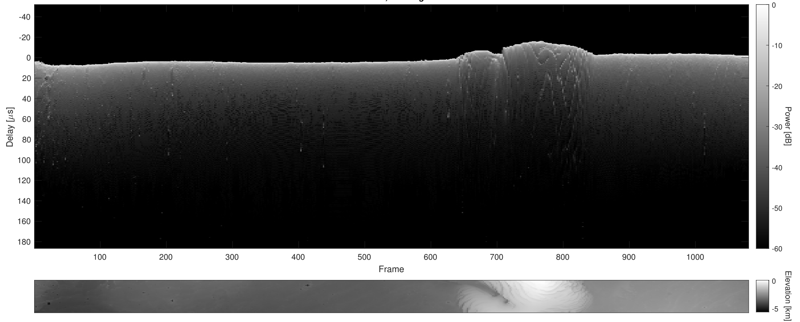
Orbit 7824, Cluttergram
