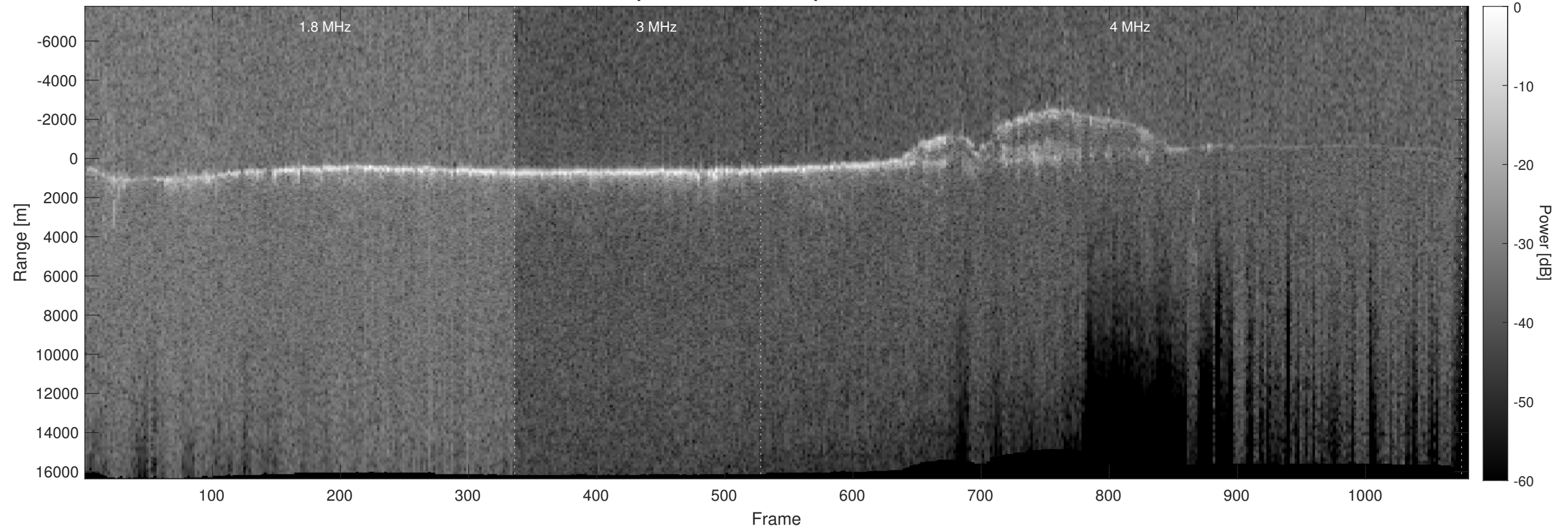
Orbit 7824, Optimized, Window, Depth-Corrected, Channel 2
