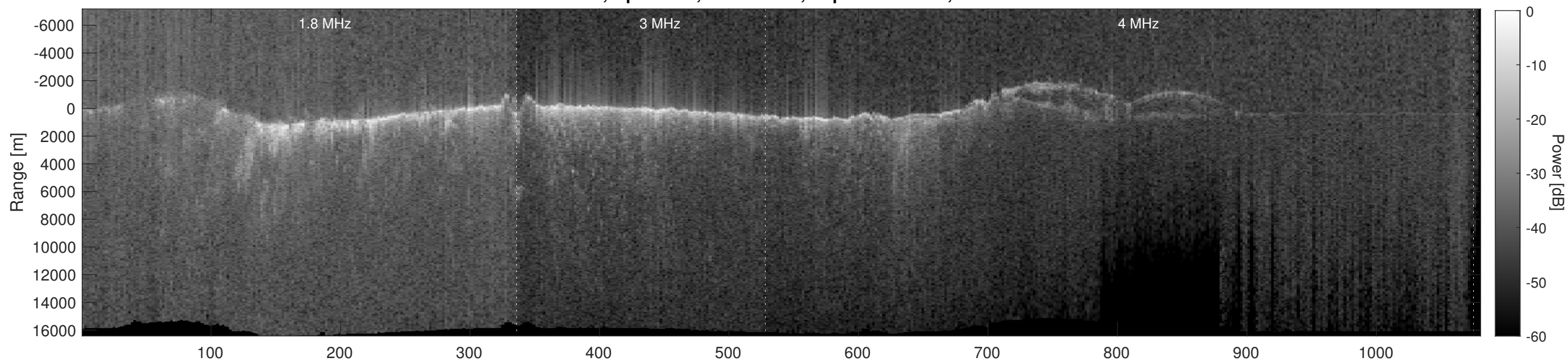
Orbit 7825, Depth-Corrected Cluttergram
