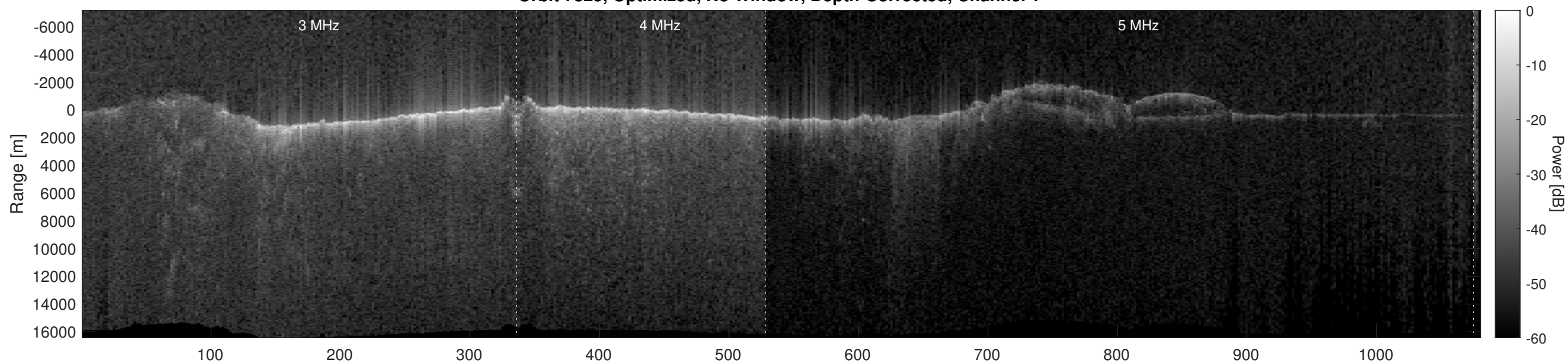
Orbit 7825, Optimized, No Window, Depth-Corrected, Channel 2
