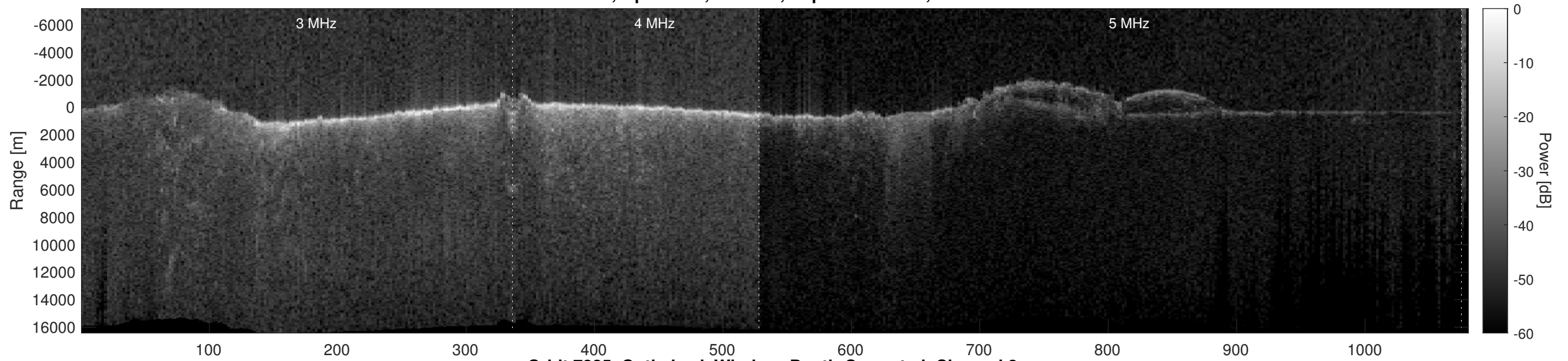
Orbit 7825, Optimized, Window, Depth-Corrected, Channel 2
