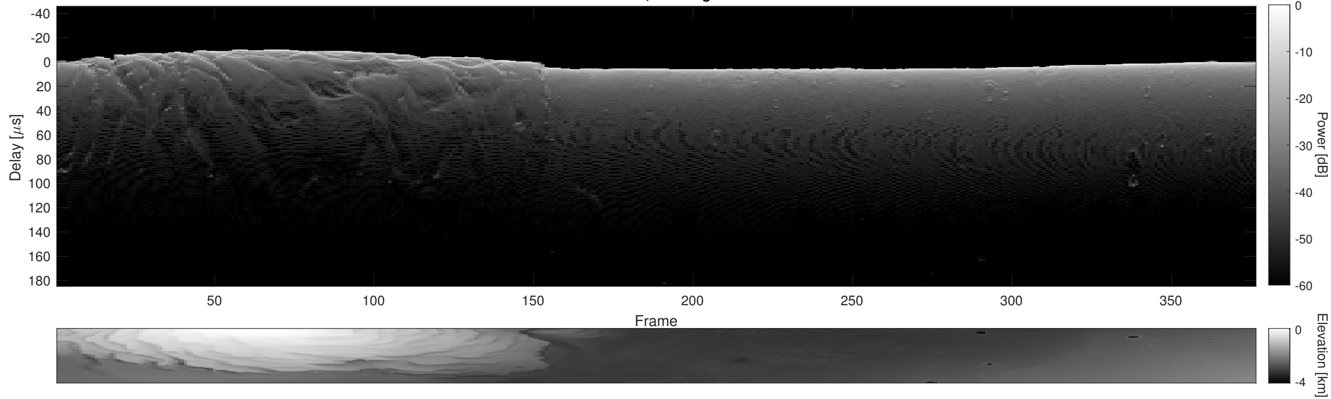
Orbit 7826, Cluttergram
