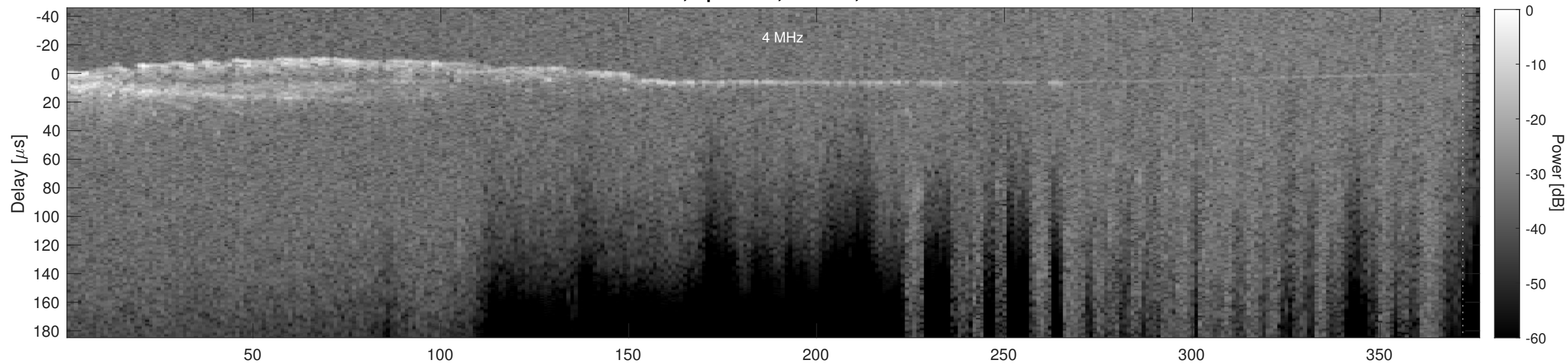
Orbit 7826, Cluttergram
