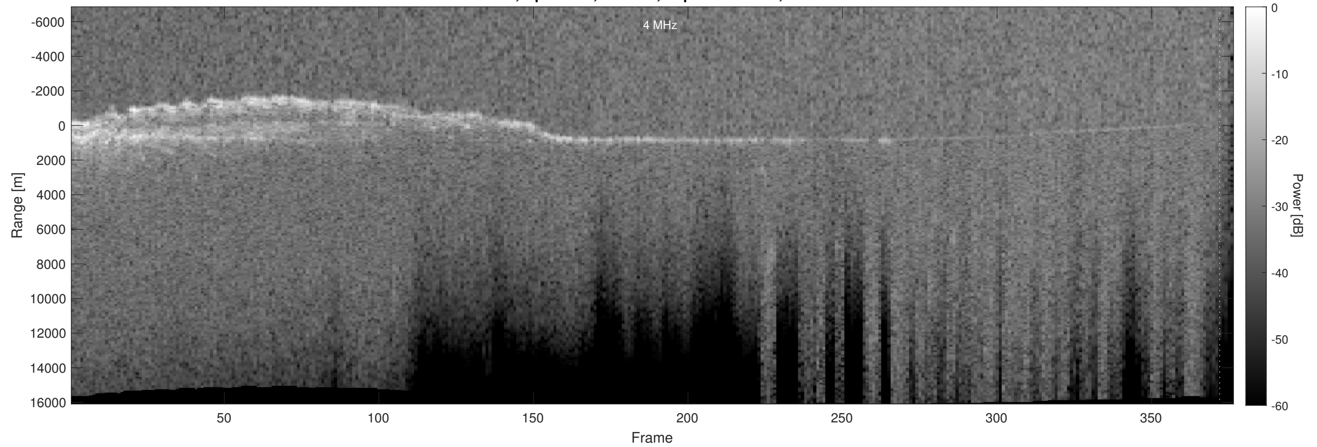
Orbit 7826, Optimized, Window, Depth-Corrected, Channel 2
