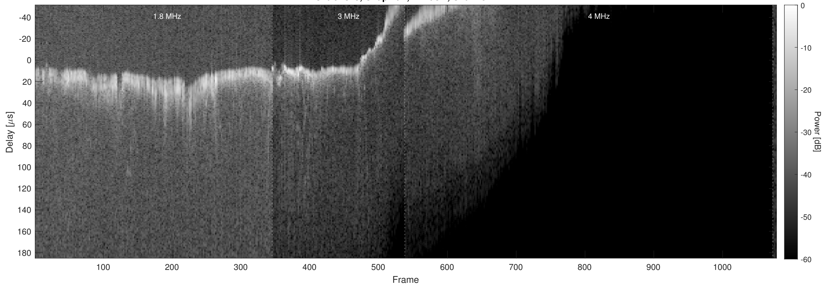
Orbit 7829, Chapman, Window, Channel 2
