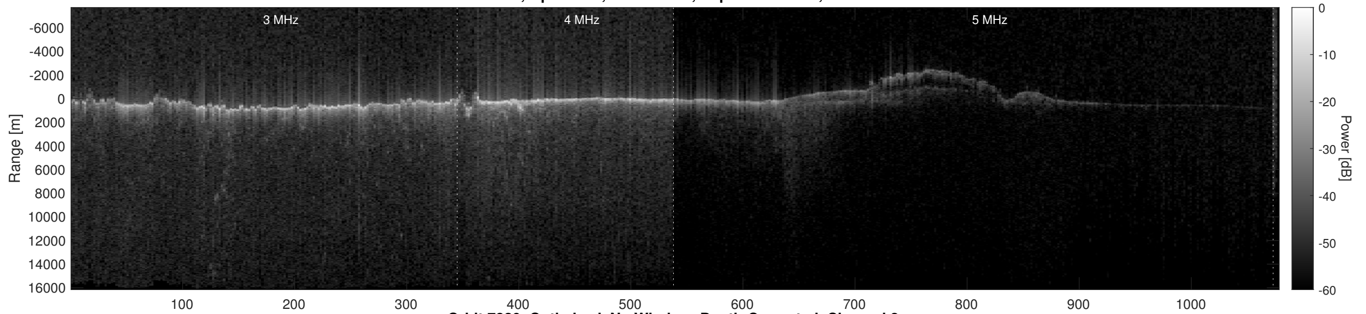
Orbit 7829, Optimized, No Window, Depth-Corrected, Channel 2
