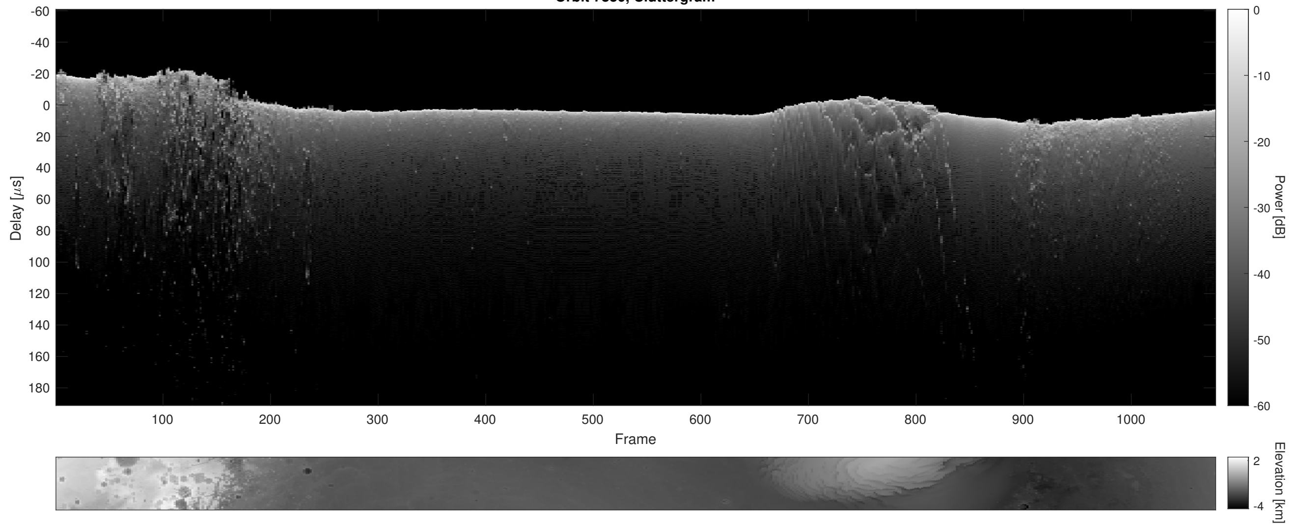
Orbit 7830, Cluttergram
