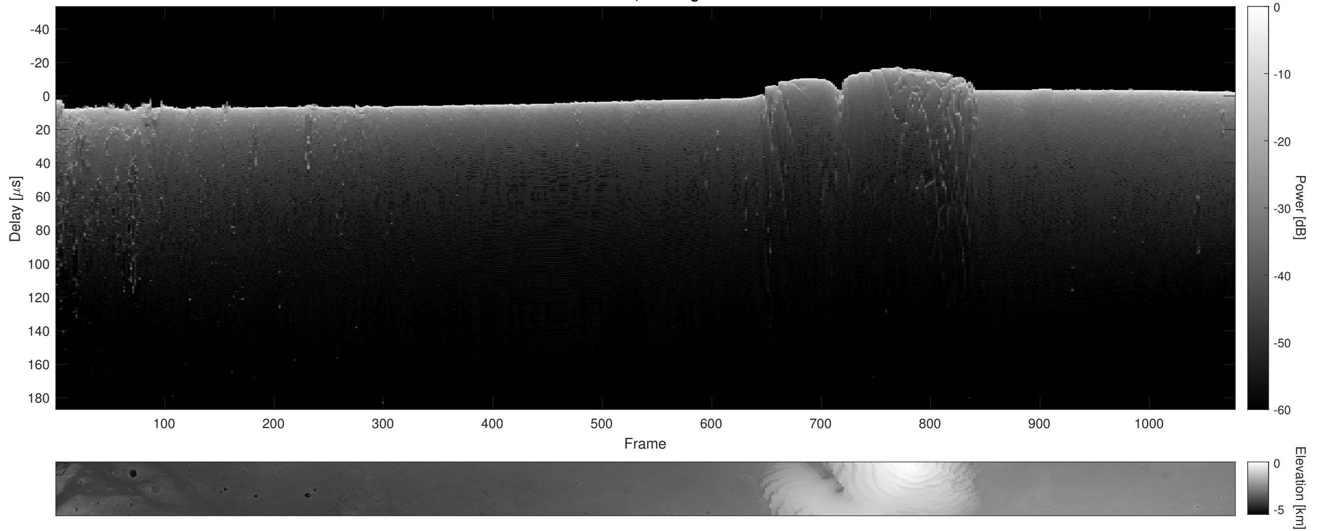
Orbit 7831, Cluttergram
