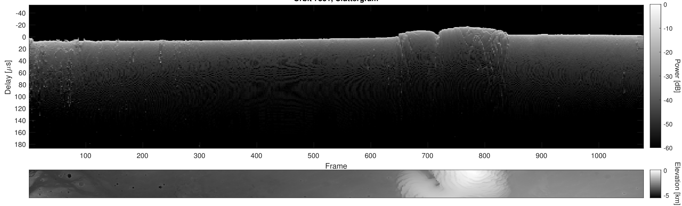
Orbit 7831, Cluttergram
