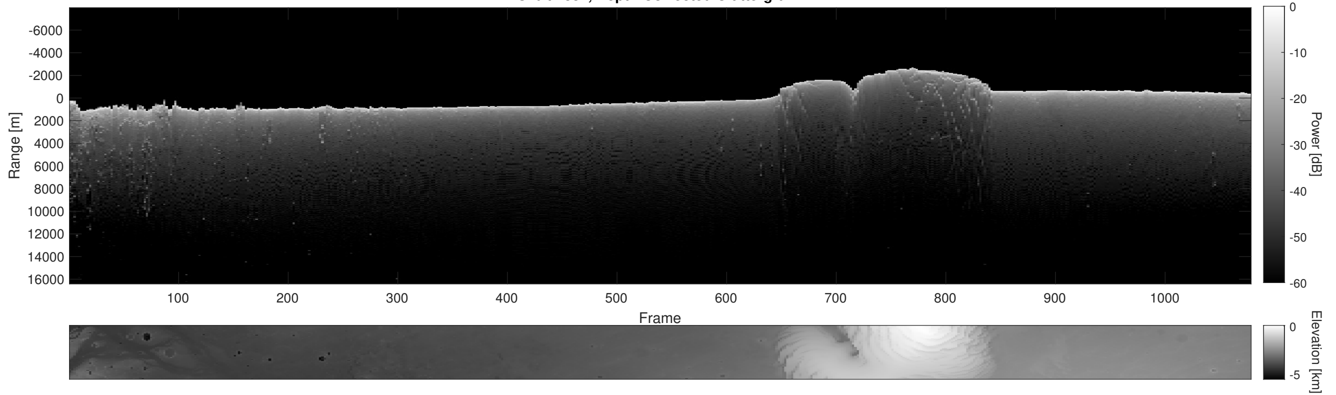
Orbit 7831, Depth-Corrected Cluttergram
