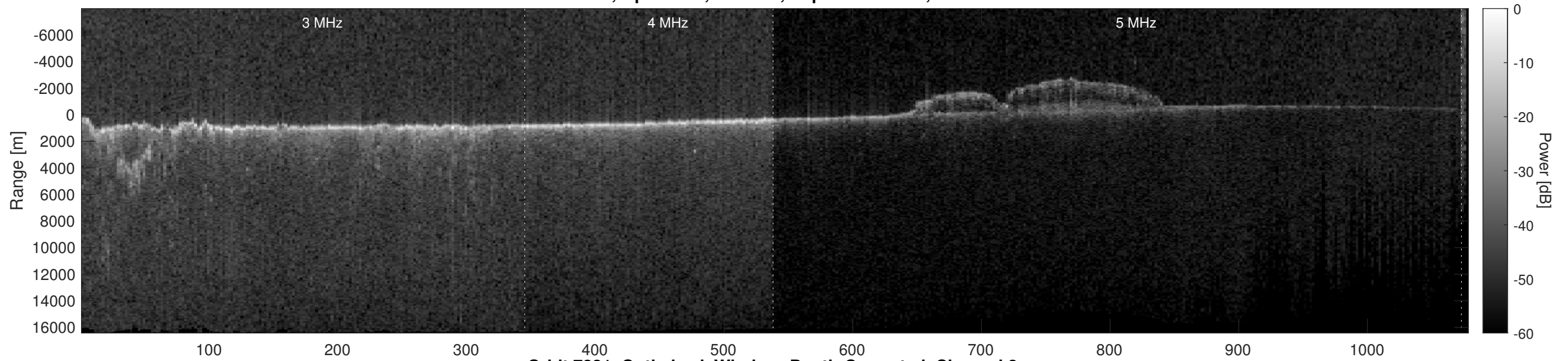
Orbit 7831, Optimized, Window, Depth-Corrected, Channel 2
