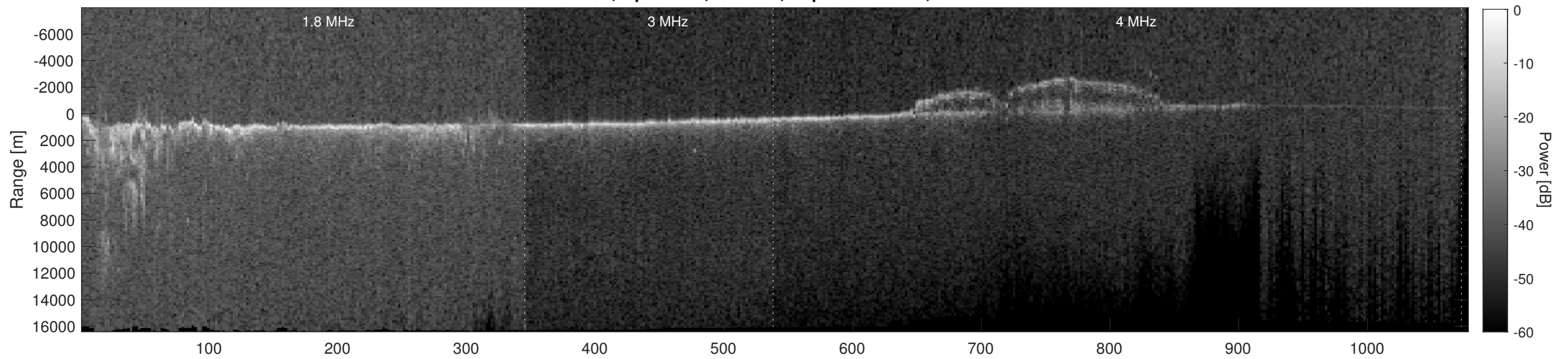
Orbit 7831, Depth-Corrected Cluttergram
