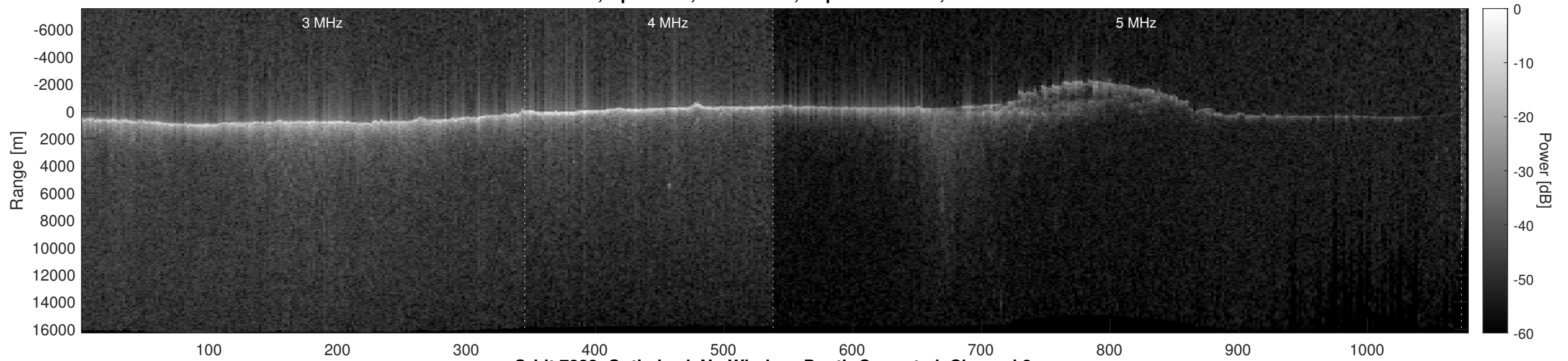
Orbit 7833, Optimized, No Window, Depth-Corrected, Channel 2
