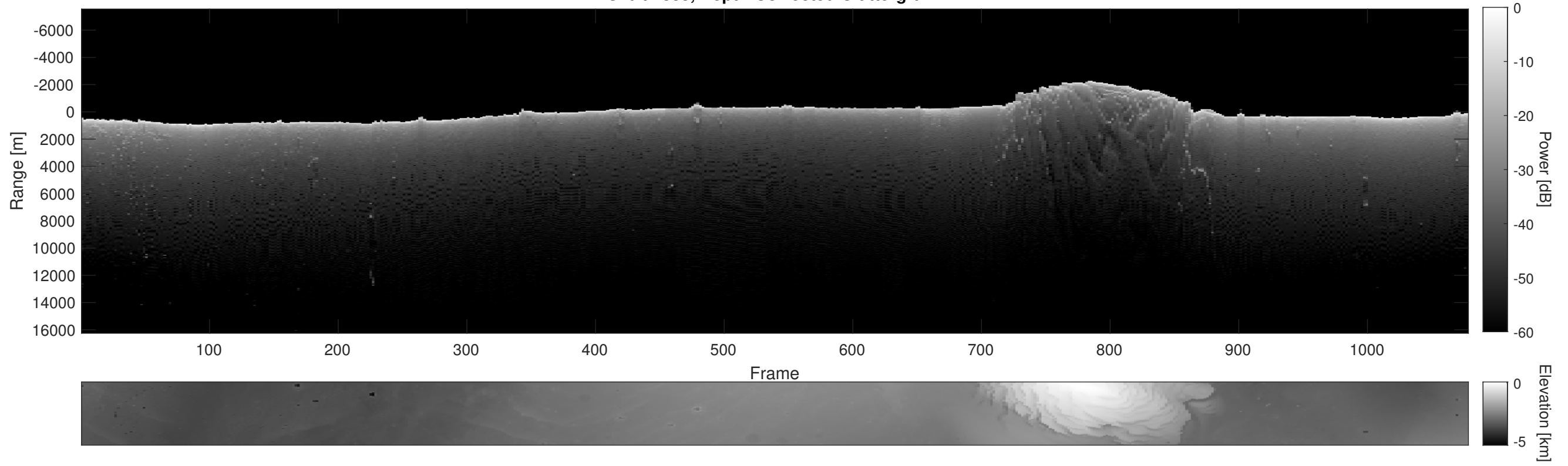
Orbit 7833, Depth-Corrected Cluttergram
