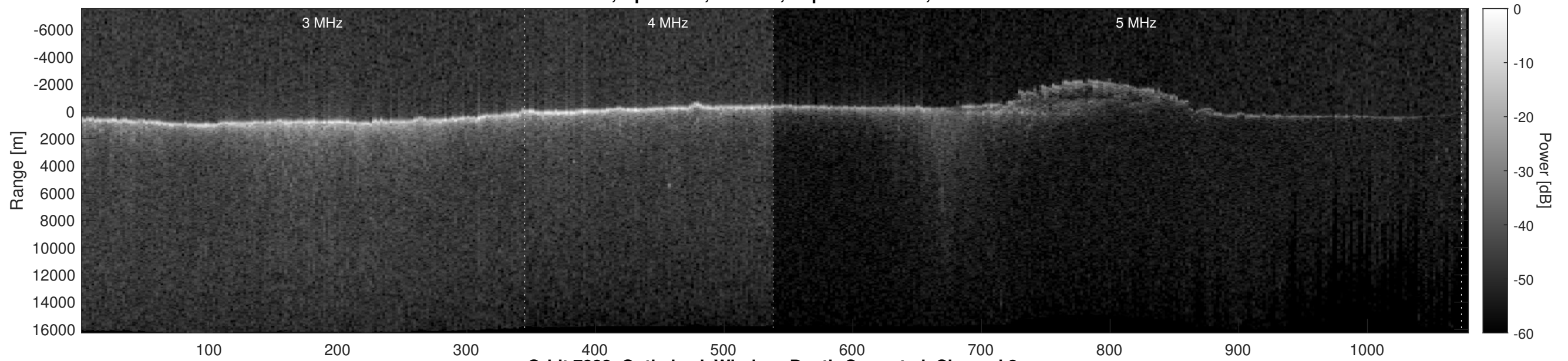
Orbit 7833, Optimized, Window, Depth-Corrected, Channel 2
