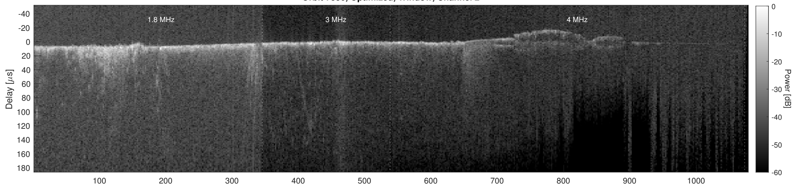
Orbit 7836, Cluttergram
