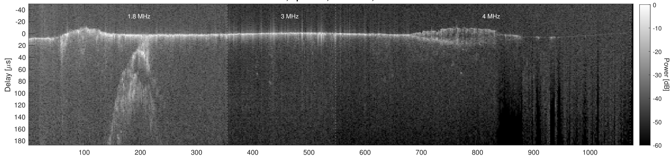
Orbit 7837, Cluttergram
