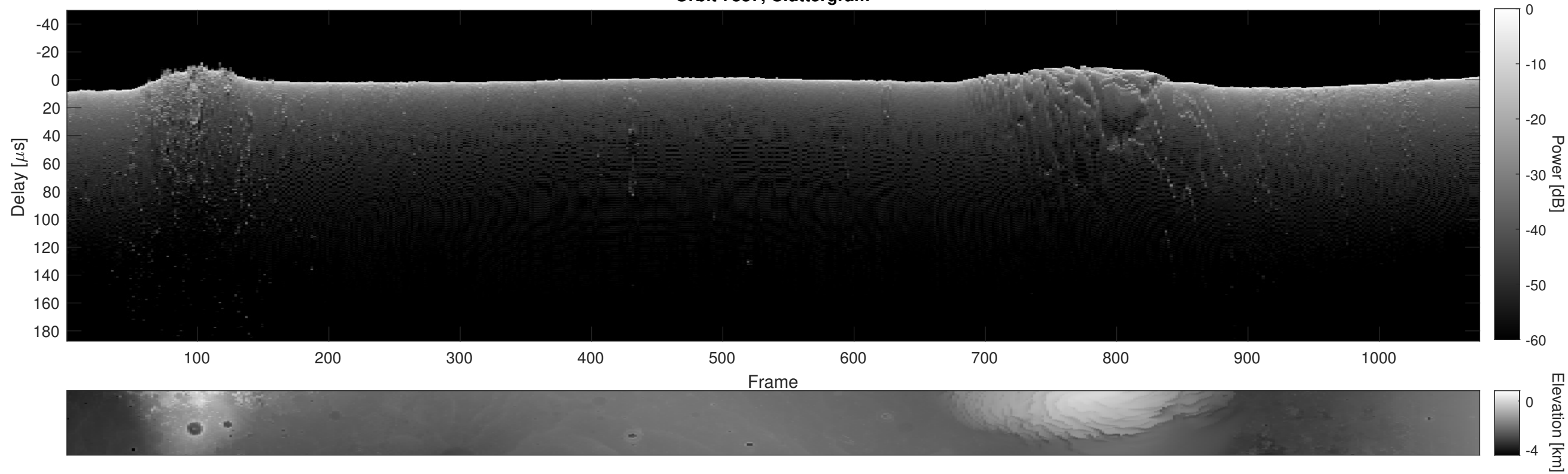
Orbit 7837, Cluttergram
