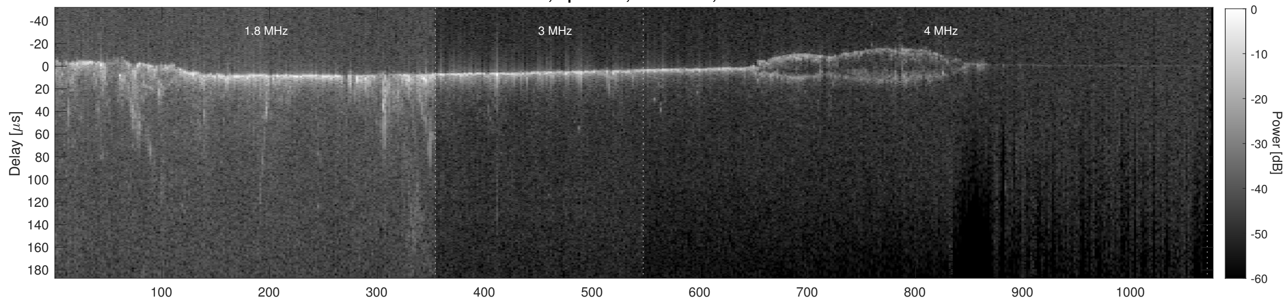
Orbit 7838, Cluttergram
