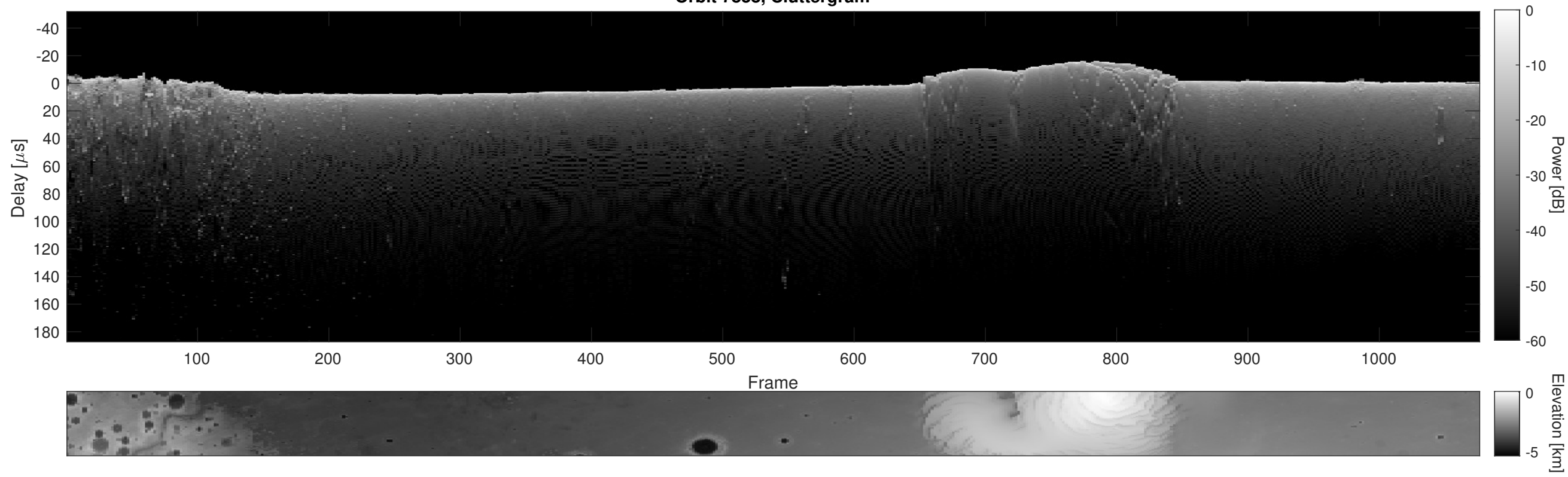
Orbit 7838, Cluttergram
