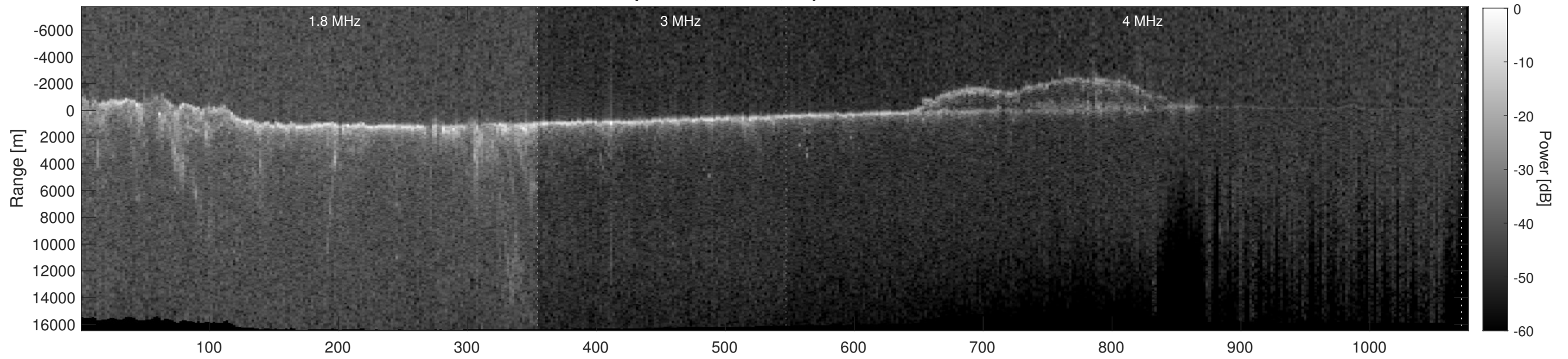
Orbit 7838, Depth-Corrected Cluttergram
