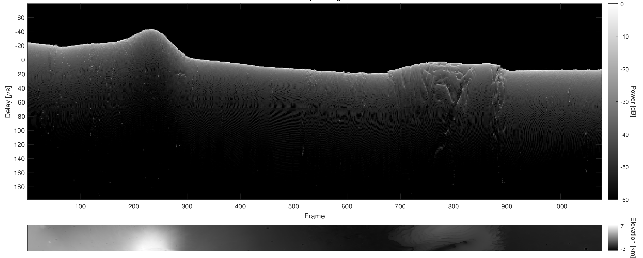
Orbit 7839, Cluttergram
