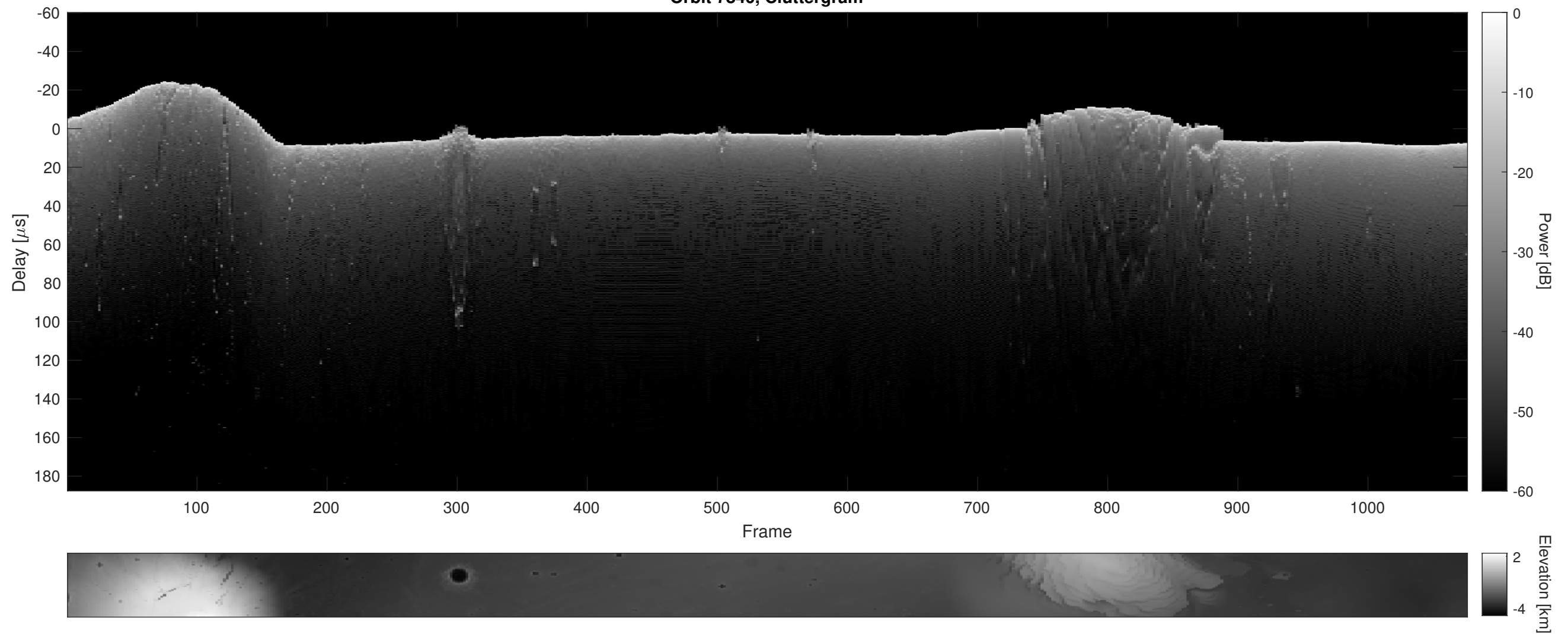
Orbit 7840, Cluttergram
