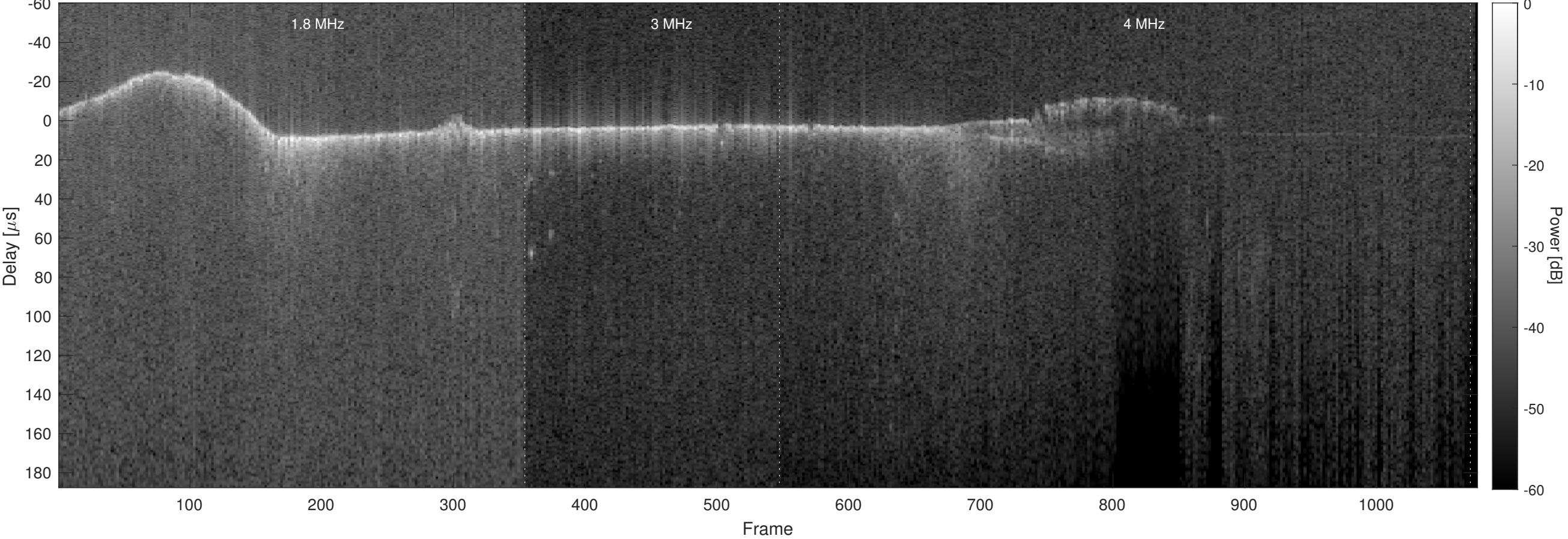
Orbit 7840, Optimized, No Window, Channel 2
