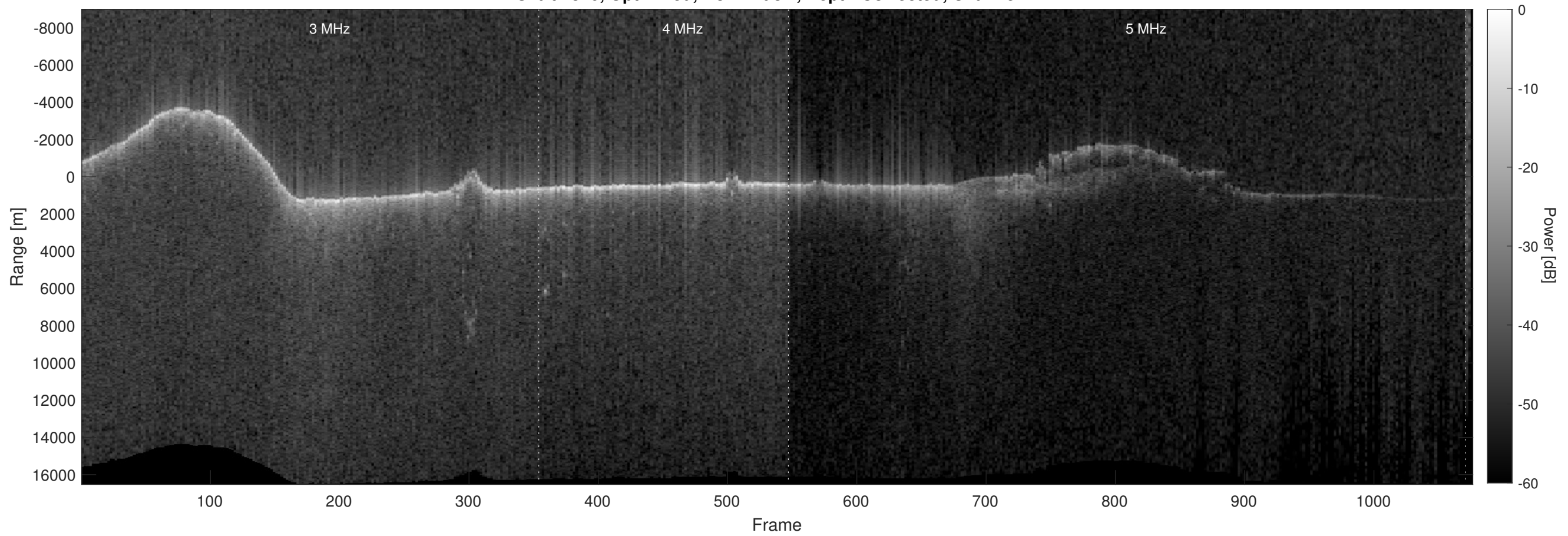
Orbit 7840, Optimized, No Window, Depth-Corrected, Channel 2
