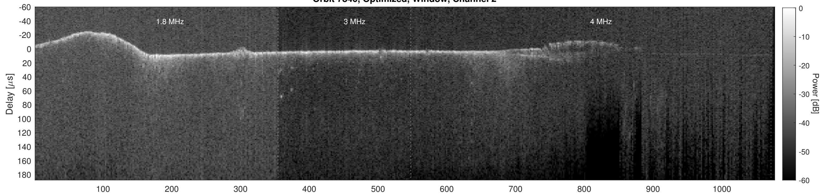
Orbit 7840, Cluttergram
