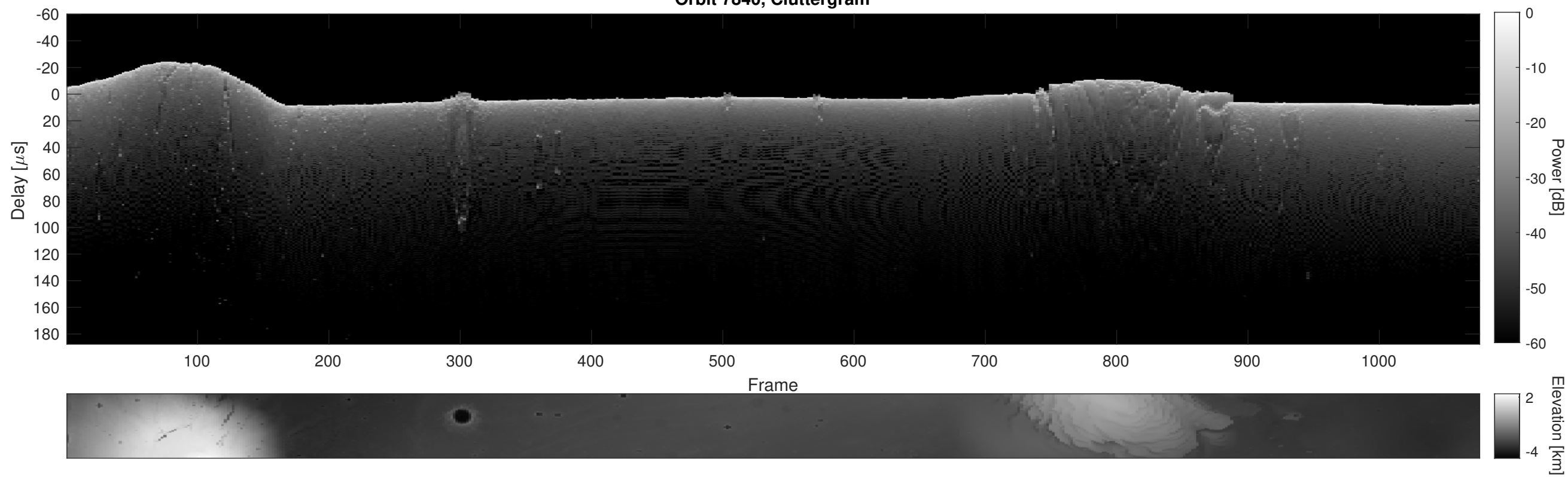
Orbit 7840, Cluttergram
