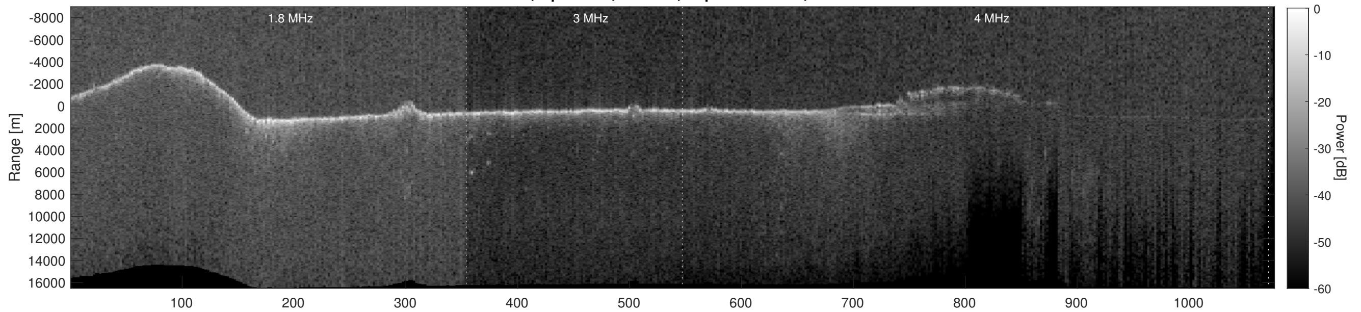
Orbit 7840, Depth-Corrected Cluttergram
