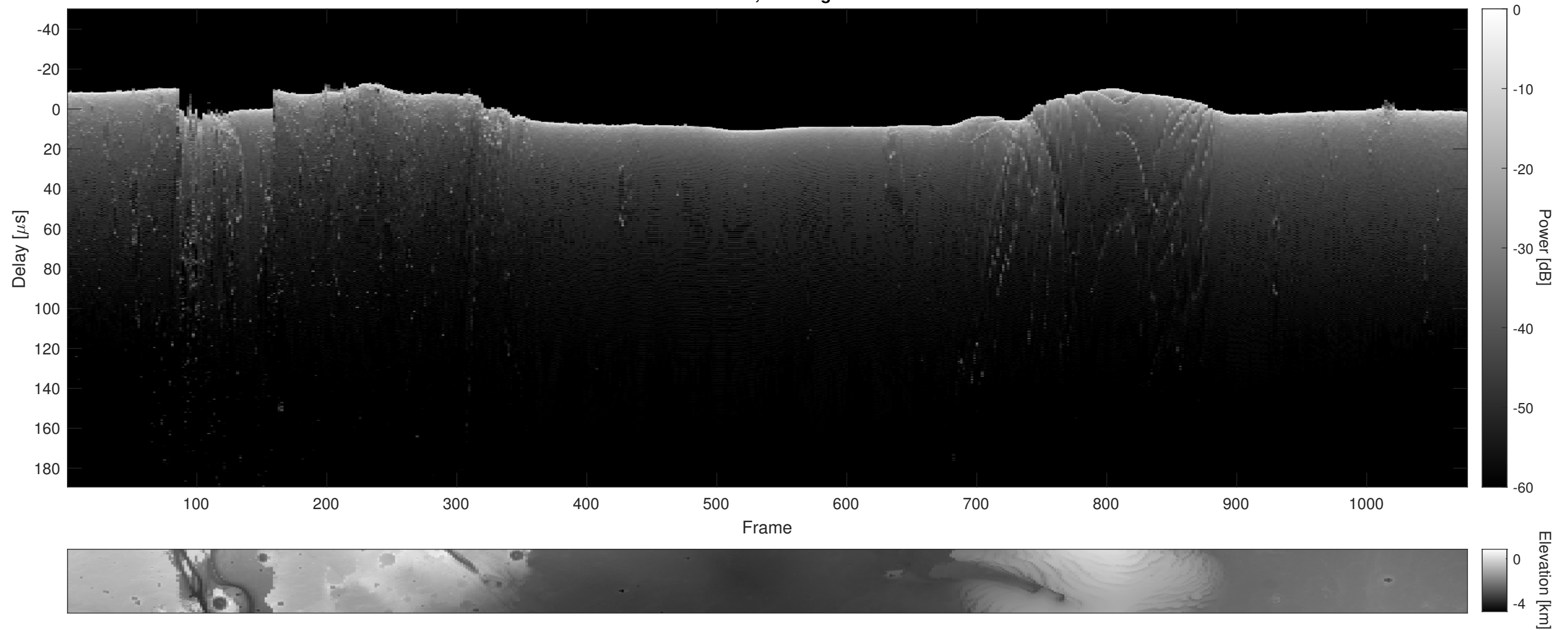
Orbit 7842, Cluttergram
