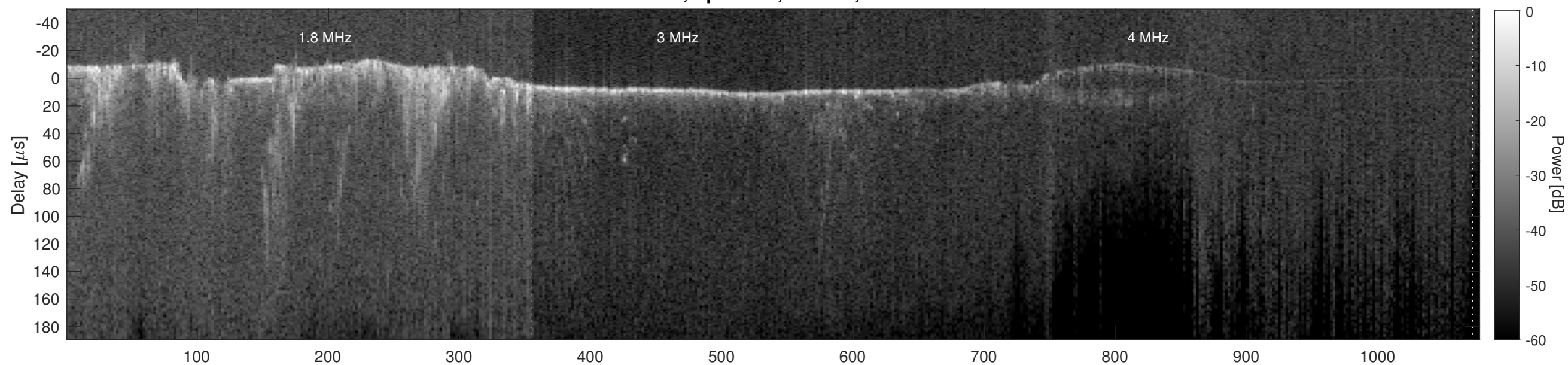
Orbit 7842, Cluttergram
