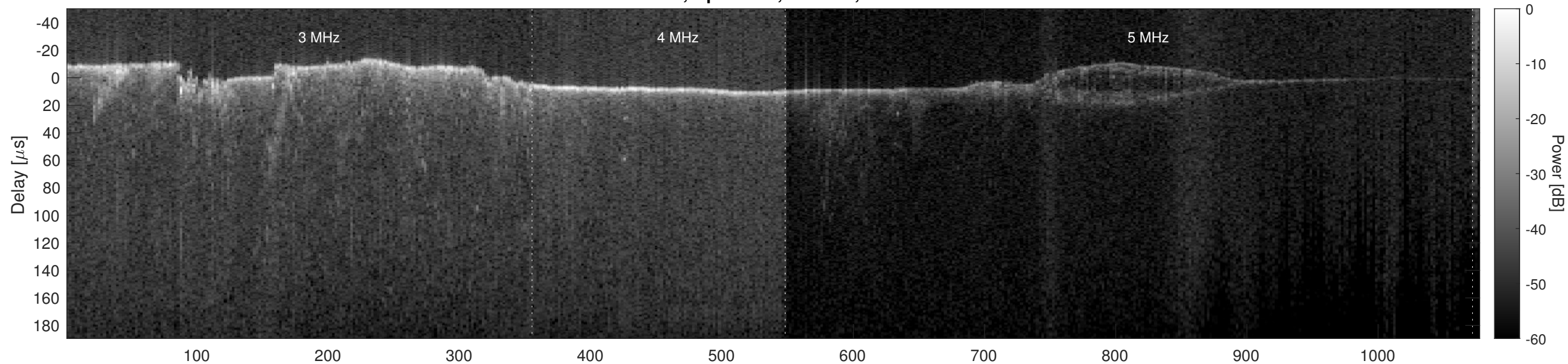
Orbit 7842, Optimized, Window, Channel 2
